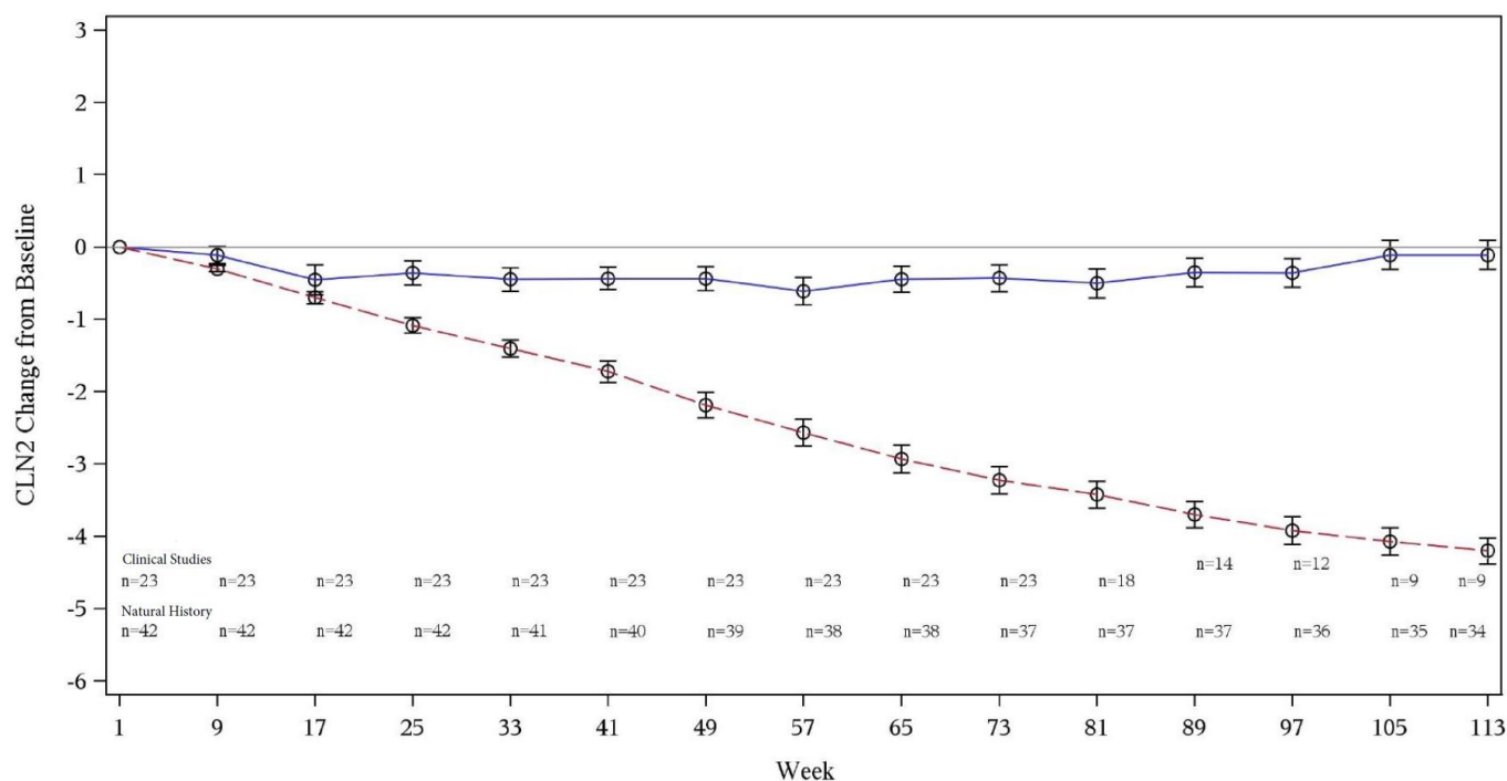
Figure 2: CLN2 Score Mean Change from Baseline (Natural History Control Group vs Brineura treated patients, 300 mg every other week)
